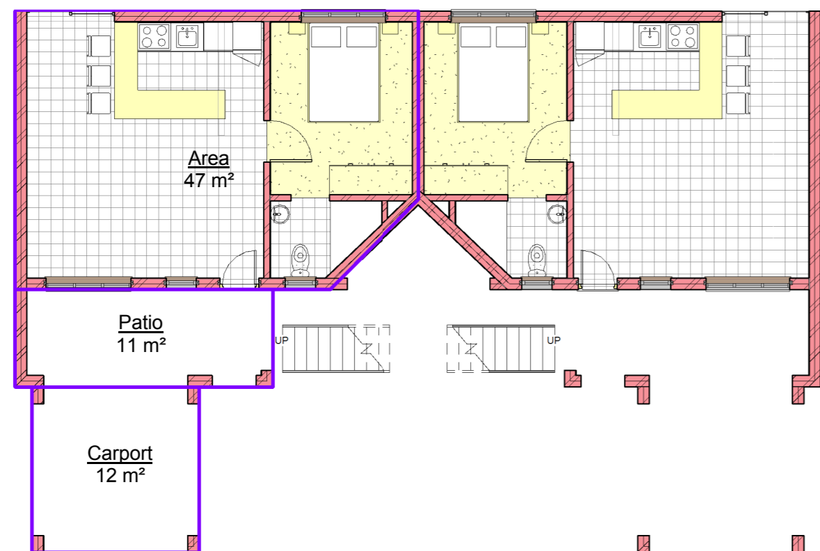
3 2 Ground Floor Bachelor Flats 1 : 100
