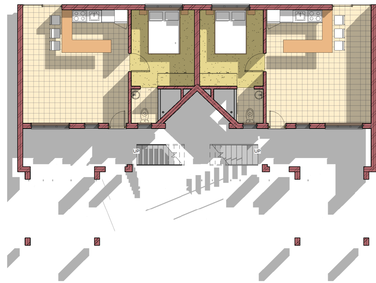
1 2 Ground Floor Bachelor Flats 1 : 100
