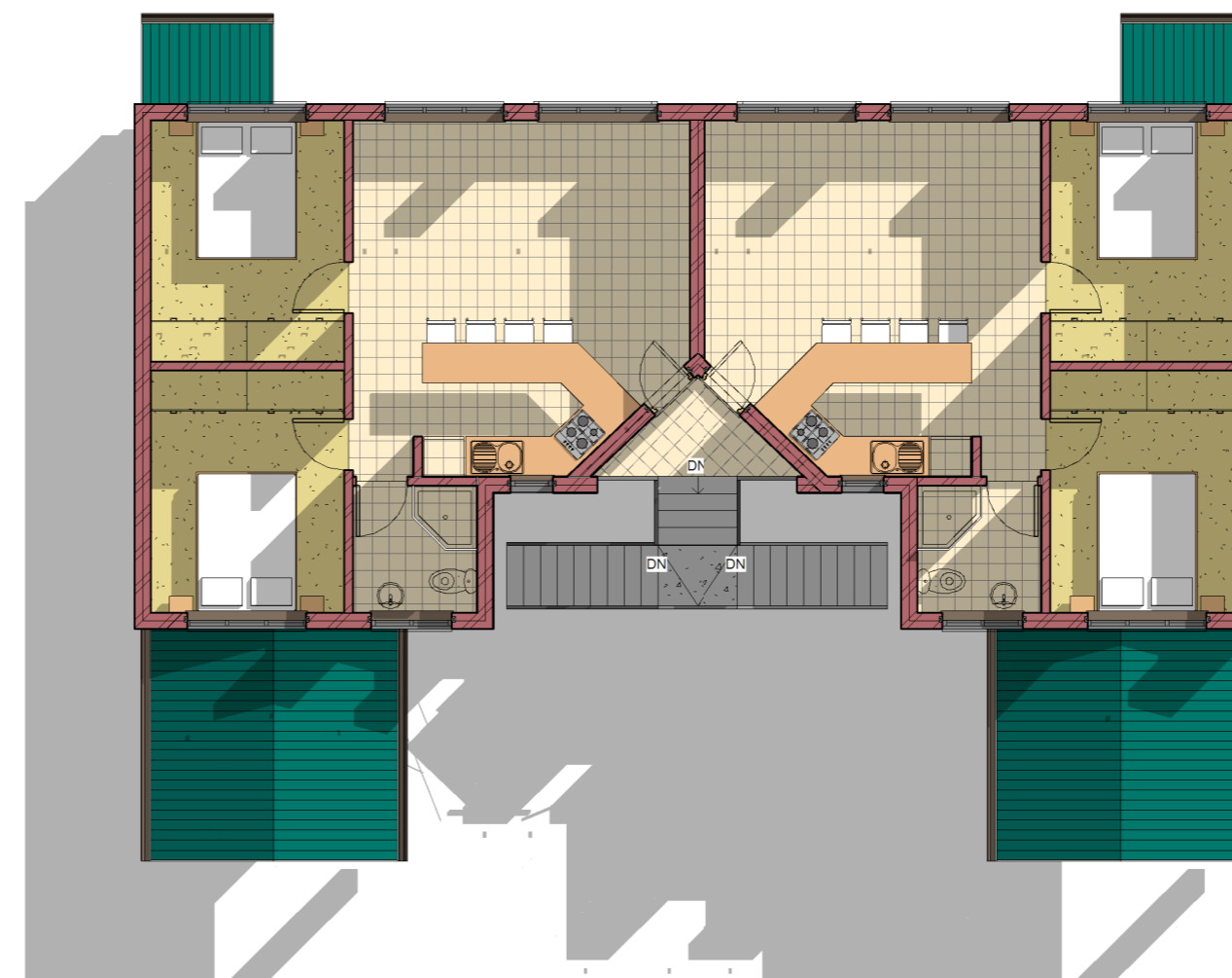
2 3 1st Floor 2 Bedroom Flats 1 : 100
