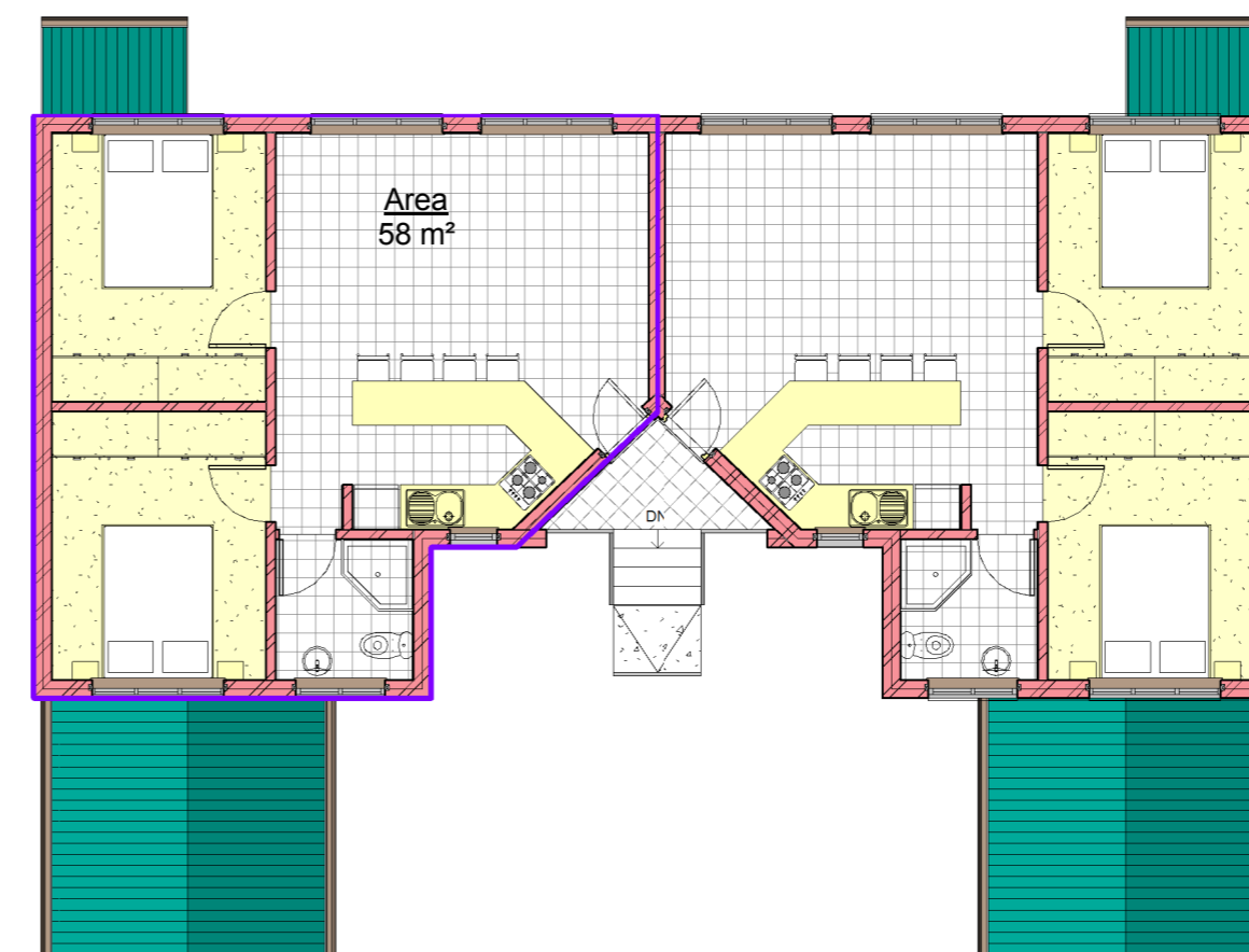
4 3 1st Floor 2 Bedroom Flats 1 : 100
